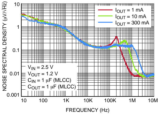
Figure 21. Output Voltage Noise Spectral Density – V OUT = 1.2 V
