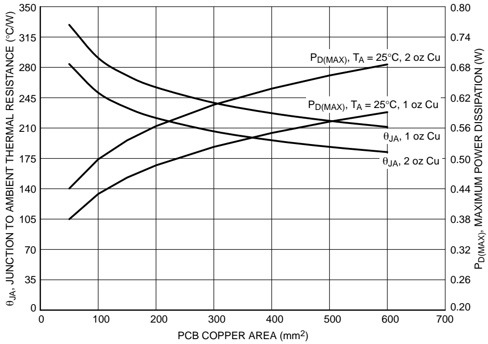
Figure 45. \theta_{JA} and P_{D(MAX)} vs. Copper Area (CSP4)
