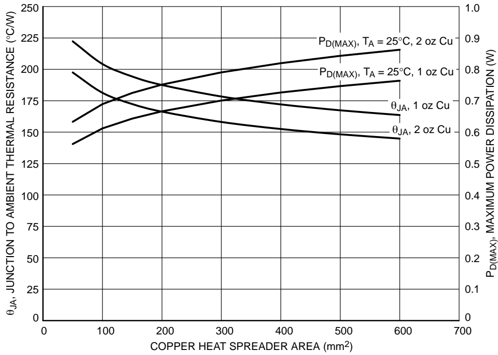
Figure 46. \theta_{JA} and P_{D(MAX)} vs. Copper Area (XDFN4)
